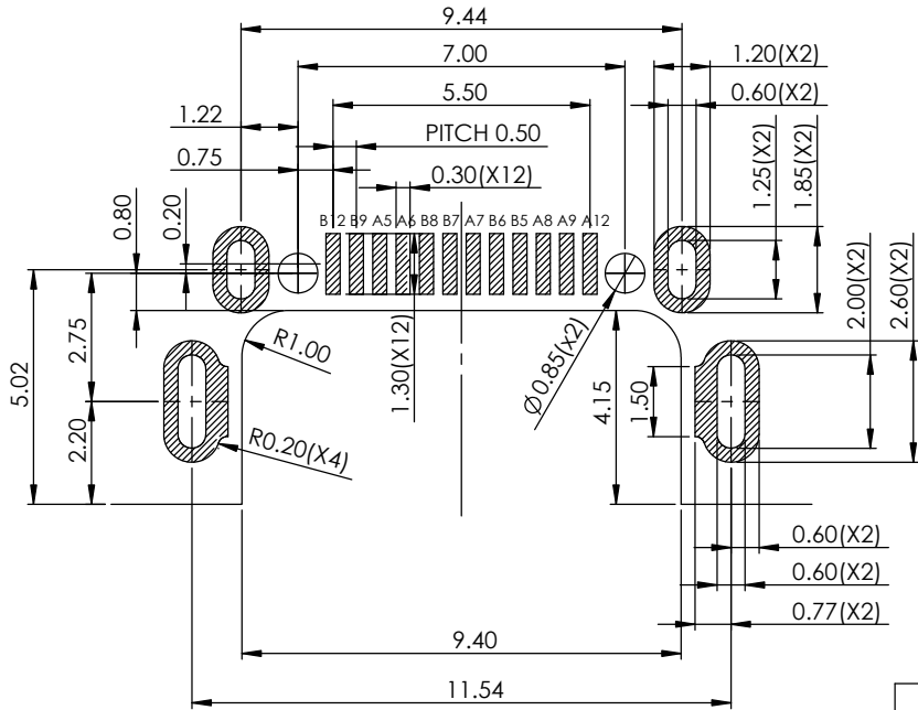
RECOMMENDED PCB LAYOUT (TOP VIEW) (TOLARANCE:±0.05)
